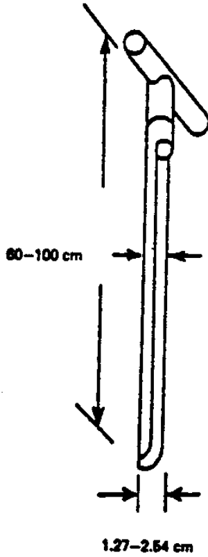
Figure 9-13. Sampling triers.
